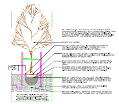
3 TREE PLANTING SCALE: 1/8"
