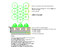
1 GROUND COVER PLANTING SCALE: 1/8"
