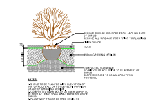
2 SHRUB PLANTING SCALE: 1/8"
