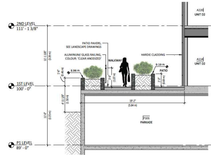
south planter section 1/4" = 1'-0"
