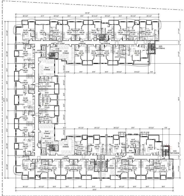
3rd - 7th level 1/16" = 1'-0"
