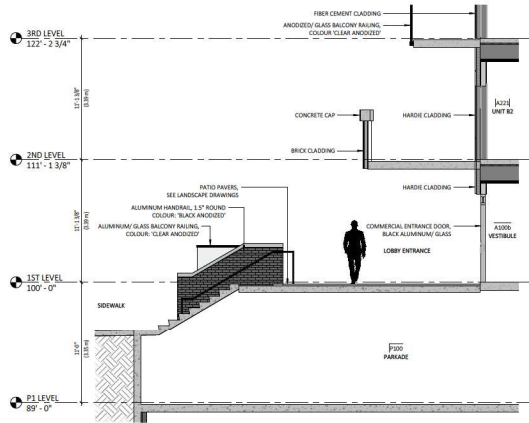
west main entry section 1/4" = 1'-0"
