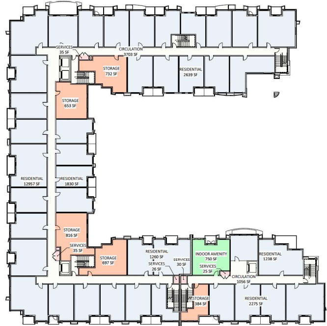
2nd level 1/16" = 1'-0"
