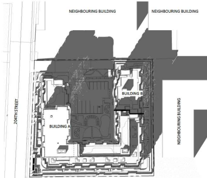
march 21-3pm 1" = 50'-0"
