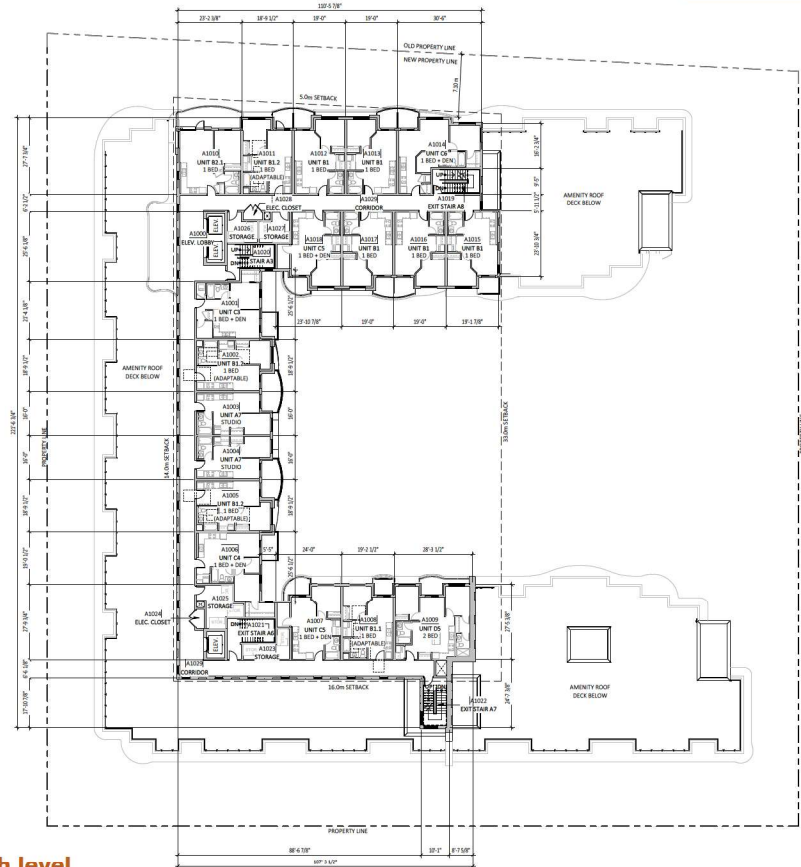
10th level 1/16" = 1'-0"
