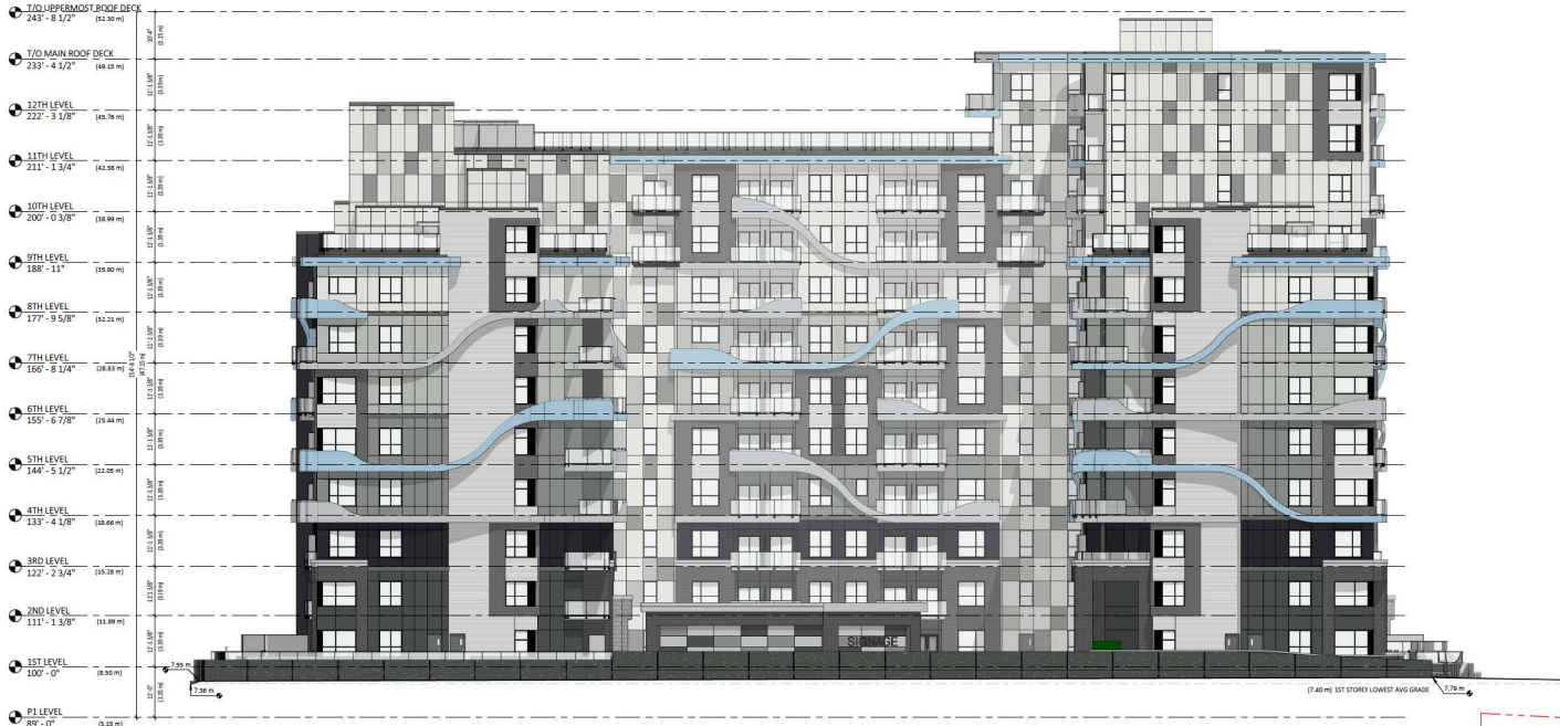
north elevation 3/32" = 1'-0"
