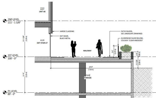
east walkway section 1/4" = 1'-0"
