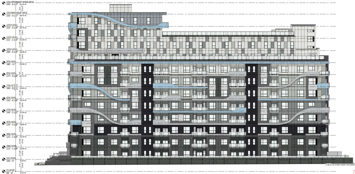
south elevation 3/32" = 1'-0"
