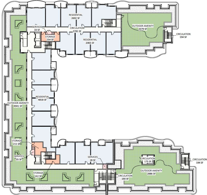
9th level 1/16" = 1'-0"
