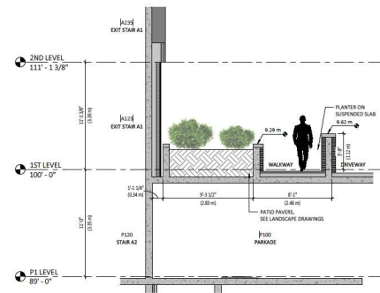
north planter section 1/4" = 1'-0"
